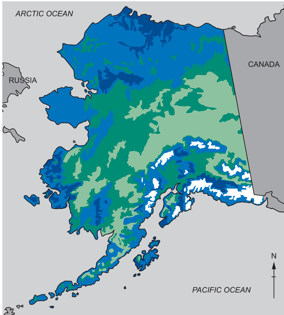
Fig. 4 – Spring snowmelt timing in Alaska 1999–2015
